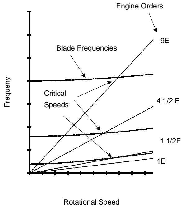
Sample Critical Speed Diagram for Engine Excitations
